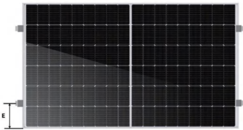
Clamps Mounting Mounting rails cross the short frame.
